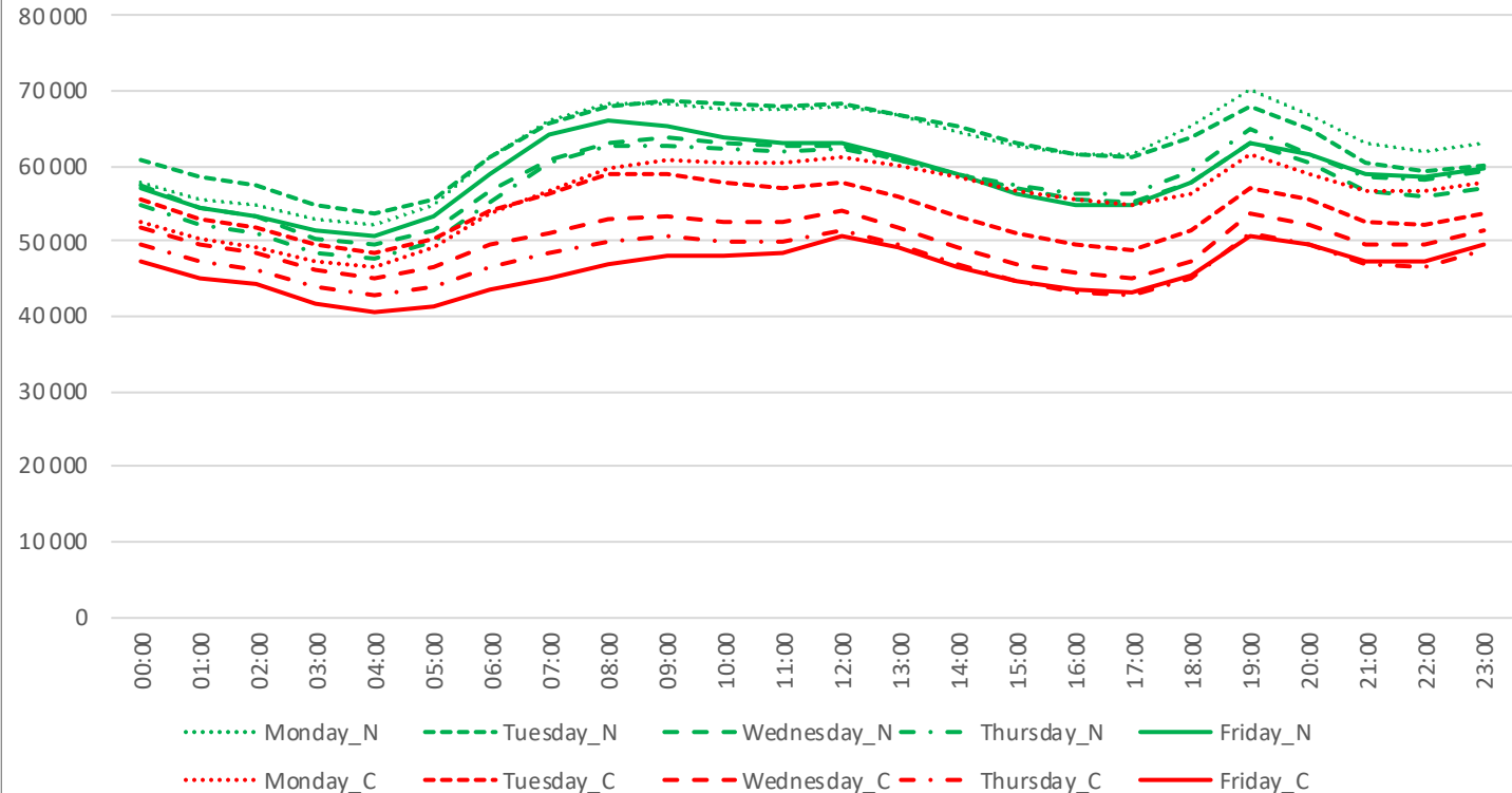
Weekday consumption for the Normal (green) and Confinement (red) week
